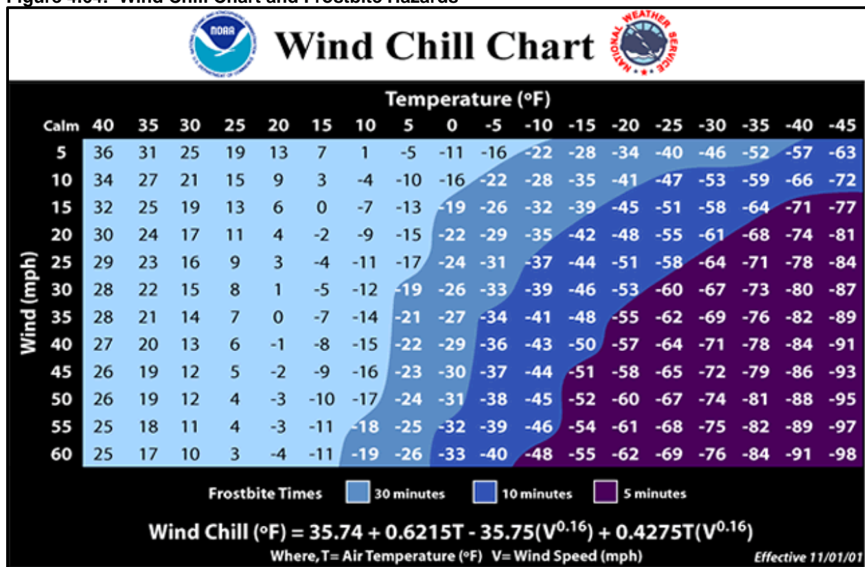
Figure 4.64: Wind Chill Chart and Frostbite Hazards
